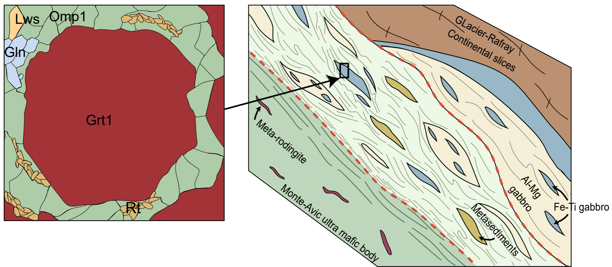
(b) M2 stage : Ca-rich fluid rock interaction, crystallization of Grt2+Omp2+Lws+Rt+ Ttn+Ap
