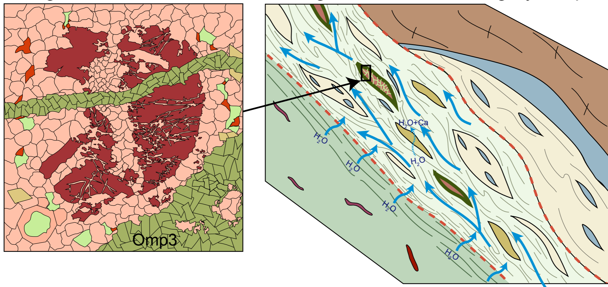
(c) M3 stage : brecciation of the former garnetite and sealing by Omp3
