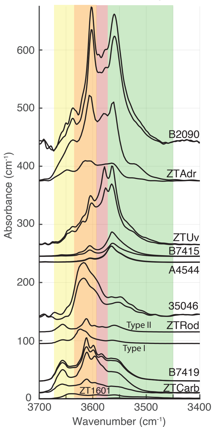
(b) Group 2 and Group 3 garnets
