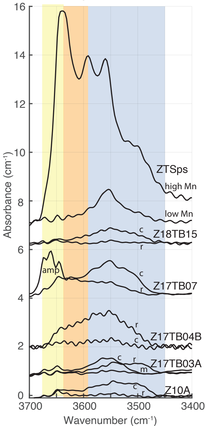
(a) Group 1 garnets
