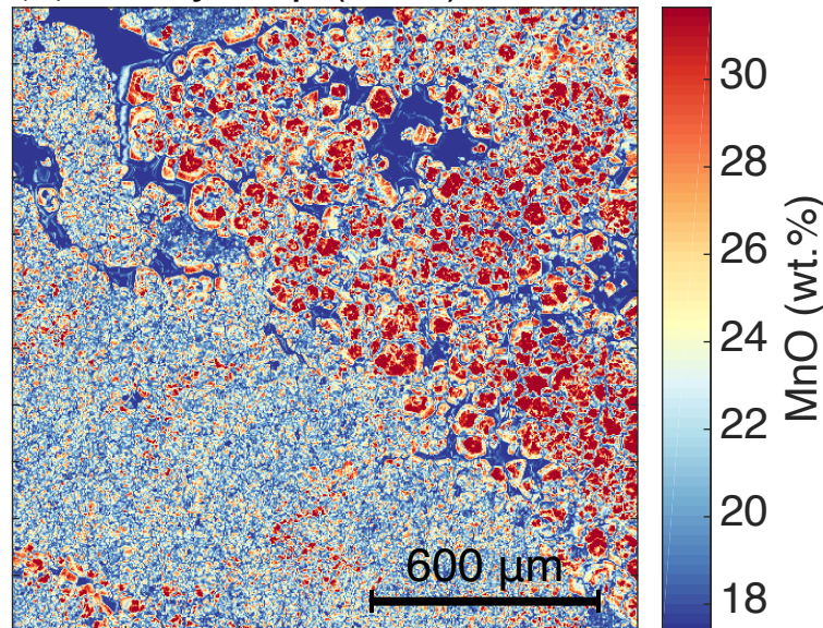
(b) X-Ray map (MnO)
