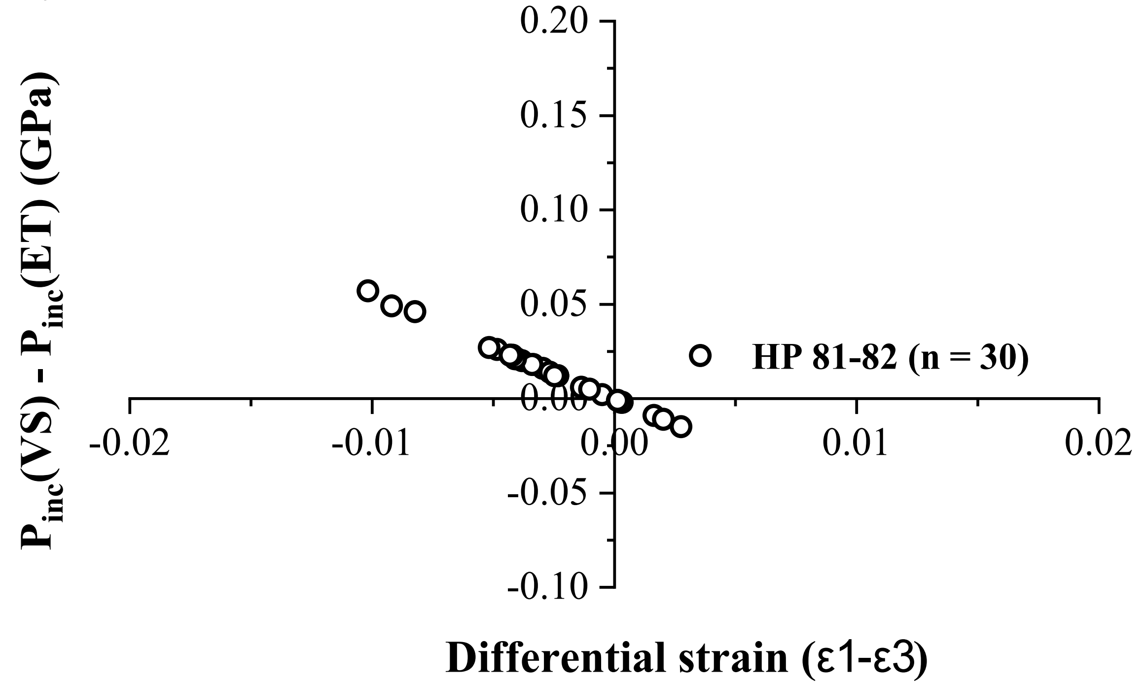
(b) P_{inc}(VS-ET) vs differential strain for iron formation inclusions
