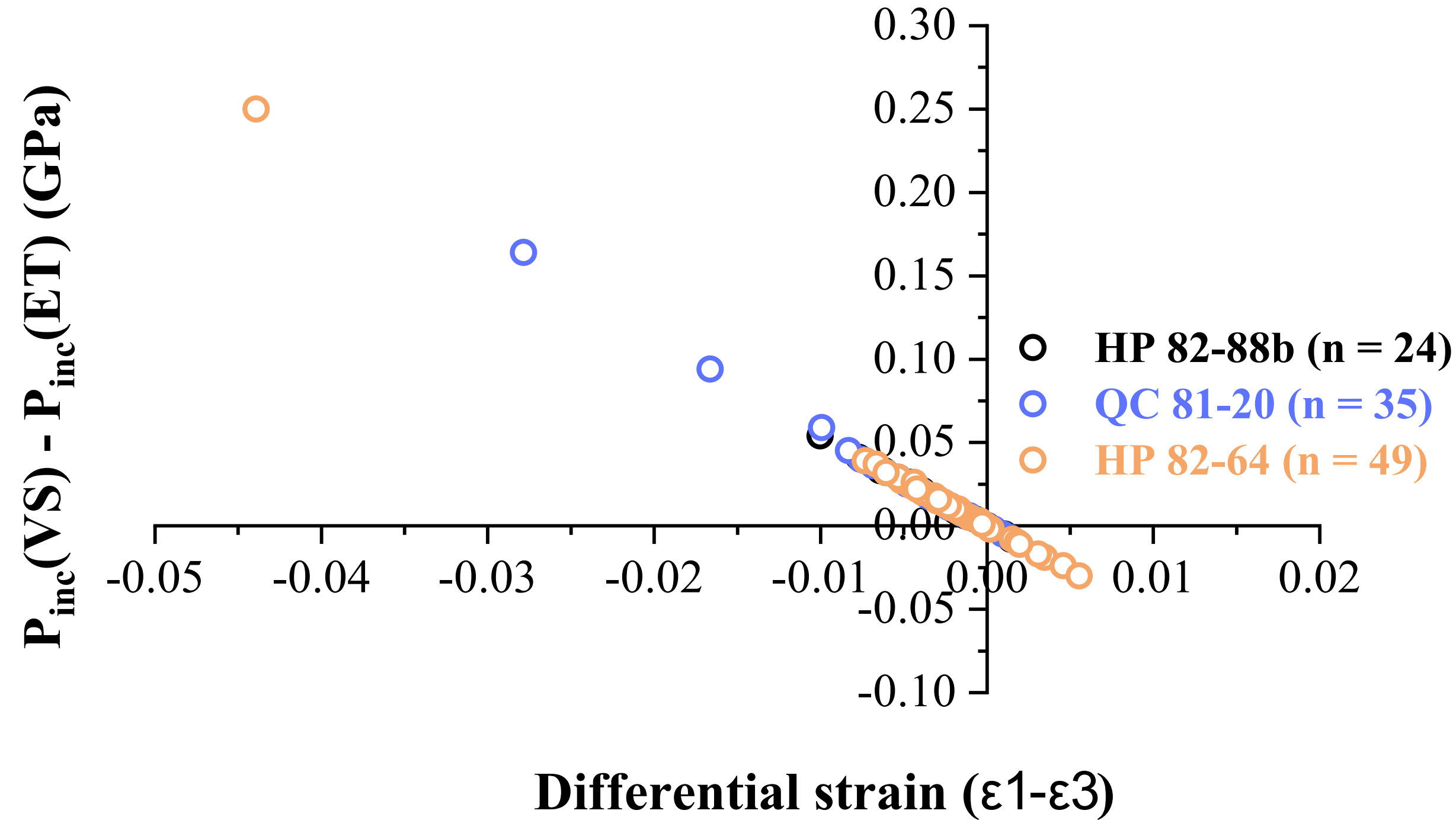
(a) P_{inc}(VS-ET) vs differential strain for migmatite inclusions
