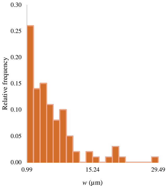
Histogram ( w )
