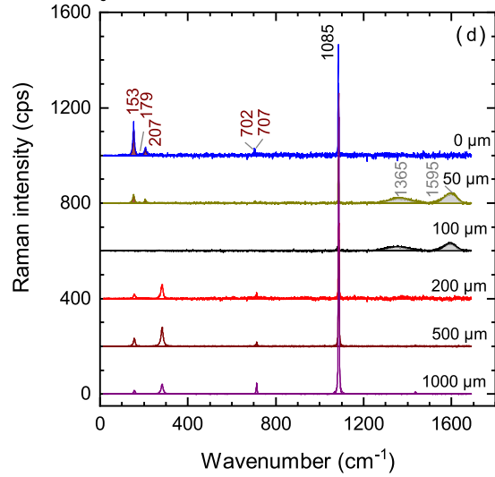
Coarse-grained (AM)
