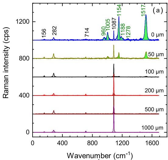
Coarse-grained (HH)
