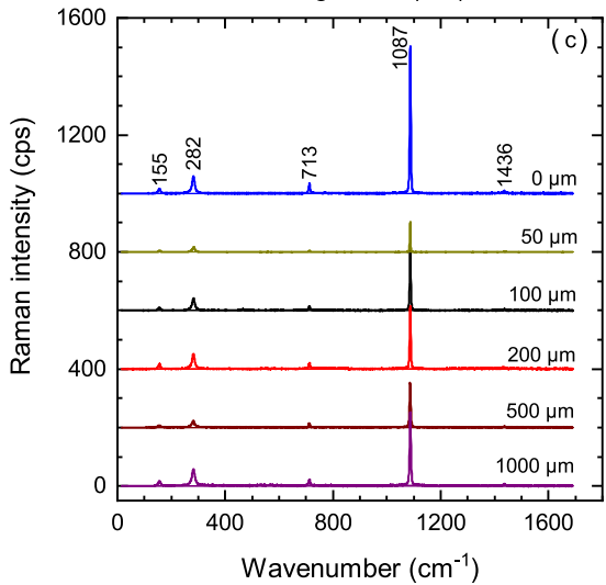
Fine-grained (HH)
